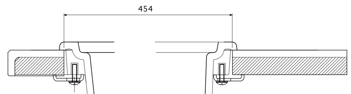
Sec B - B
